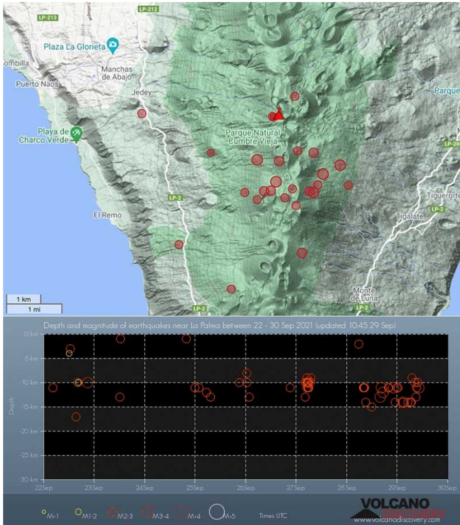
Earthquakes under La Palma during the past 48 hours
